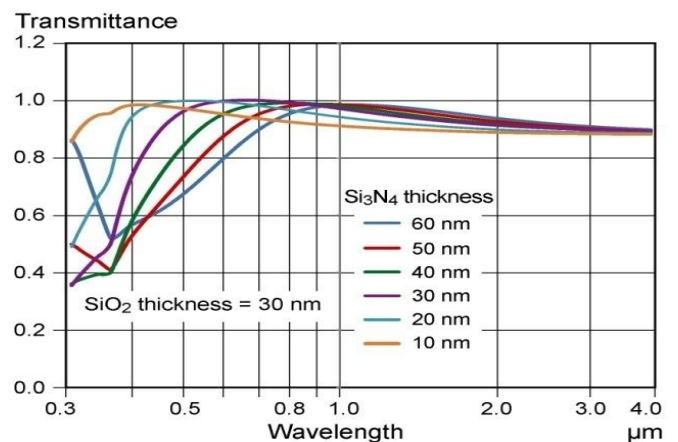
Fig. 4. Spectral dependence of optical transmission for different thicknesses of silicon nitride
