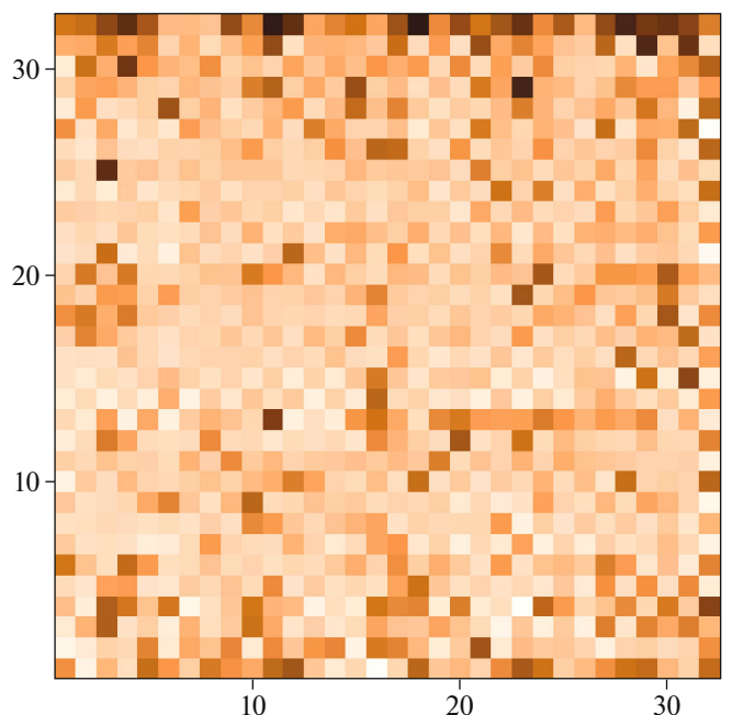
Fig. 6. Required image of 32 \times 32 points given by the infrared 32 \times 32 FPA uniformly illuminated by the IR-source (blackbody simulator) at temperature 50^\circ\text{C} . Each point represents a response from the corresponding bimaterial IR-detector (points are depicted as squares). The image was obtained as a result of computer processing conducted according to the FOS method. The dark points correspond to strongly deformed membranes of the bimaterial IR-detectors.
