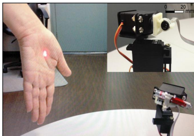
Figure 3. Scanning system with HTPA4x16 module performing the functions of detection, capture and tracking of a moving thermal object (fragment of video)
